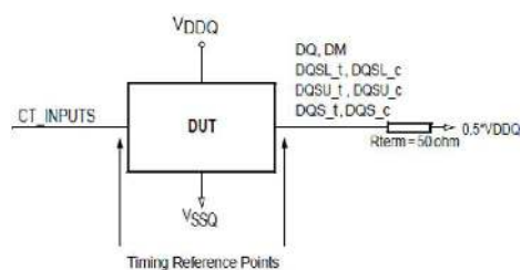
Connectivity Test Mode Timing Reference Load
